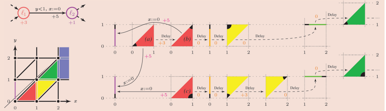
Figure 4. The corner-point abstraction refines the region abstraction by also keeping track of the corner point close to which an execution runs. This is needed to measure costs: for instance, if we are in location \ell_1 and in the red region where 0 < y < x < 1 , the price of delaying depends on the value of the clocks. From (a), where both x and y are arbitrarily close to 0, we can let almost one time-unit elapse and reach (b). The resulting cost is arbitrarily close to +3. On the other hand, from (c), where x and y are arbitrarily close to 1 and 0, respectively, letting time elapse takes us to the subsequent region, so that the cost is arbitrarily close to 0. (Notice that for readability, some resetting transitions have been omitted.)
