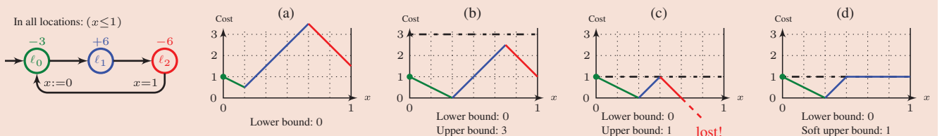
Figure 5. The resource management problem asks whether it is possible to maintain the cost level within fixed bounds. There can be a lower bound only (a), a lower and an upper bound (b, c), or a lower bound and a soft upper bound above which cost level cannot increase. Figures (a), (b), and (d) represent solutions to the respective problems for the priced timed automaton depicted on the left: there is an infinite run that satisfies the global constraint. In case (a) for instance, we have depicted a possible schedule for the first cycle, and this run can be repeated because at the start of the second cycle, the cost level is larger than at the start of the first cycle. In Figure (c), the proposed schedule violates the lower bound, and it can be shown that there exists no infinite run which maintains cost level within the specified bounds.
